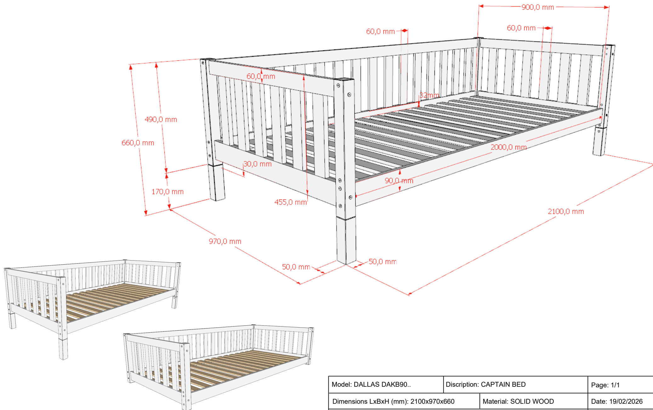
CAPTAIN BED WITH REMOVABLE LEGS TO MAKE A FLOORBED
